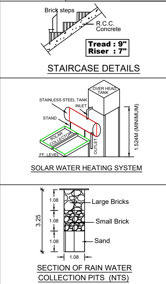
SECTION OF RAIN WATER COLLECTION PITS (NTS)
