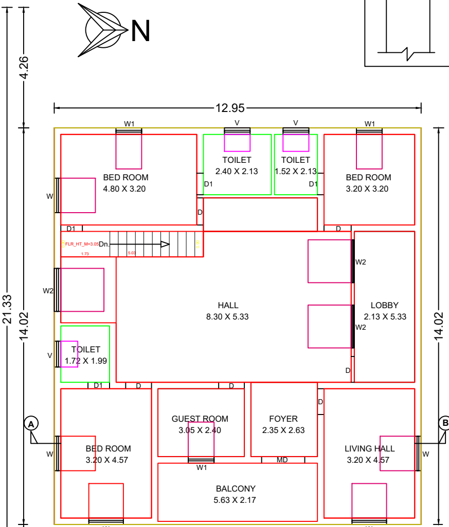
FIRST FLOOR PLAN (PROPOSED)
