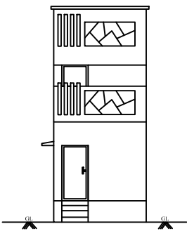
FRONT ELEVATION
