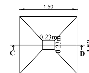
SECTION - 'CD'
