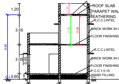
SECTION ON SS
