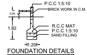
FOUNDATION DETAILS
