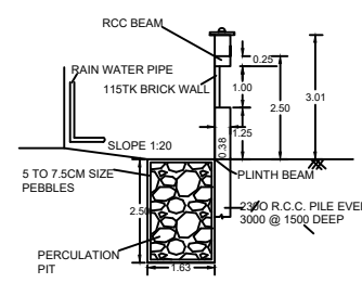
RAINWATER HARVESTING
