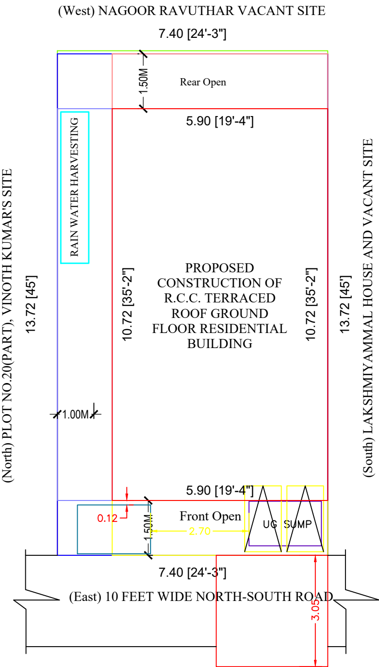
SITE PLAN
