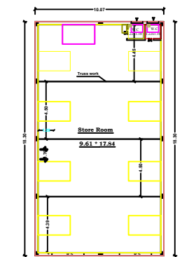
Proposed Ground Floor Plan - Store Room
