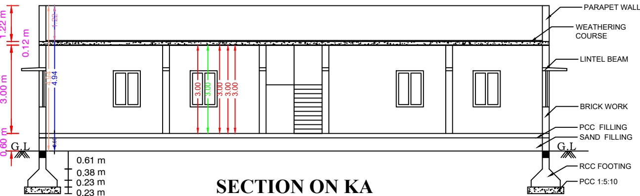
SECTION ON KA
