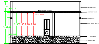
SECTION ON K-S
