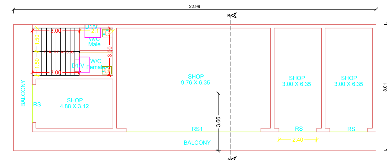
PRO.GROUND FLOOR PLAN
