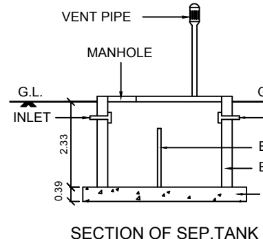
SECTION OF SEP.TANK
