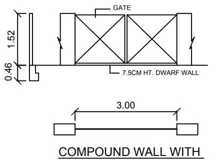
COMPOUND WALL WITH DWARF WALL DETAILS
