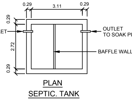
PLAN SEPTIC TANK
