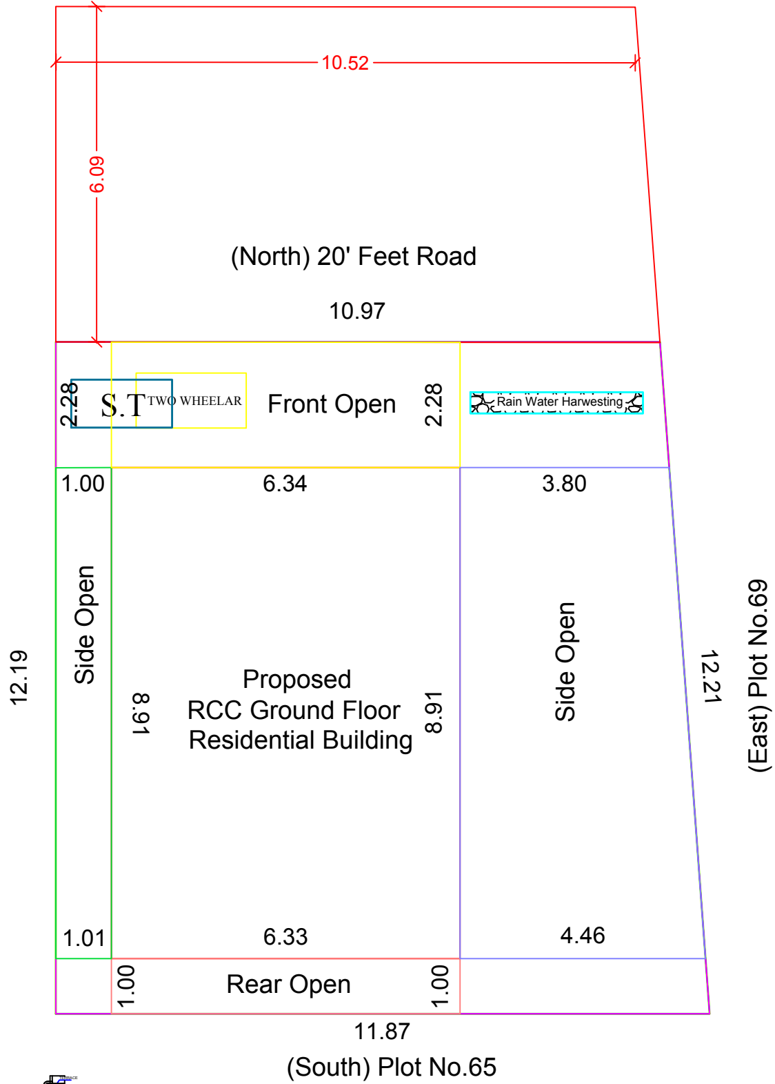
SITE PLAN
