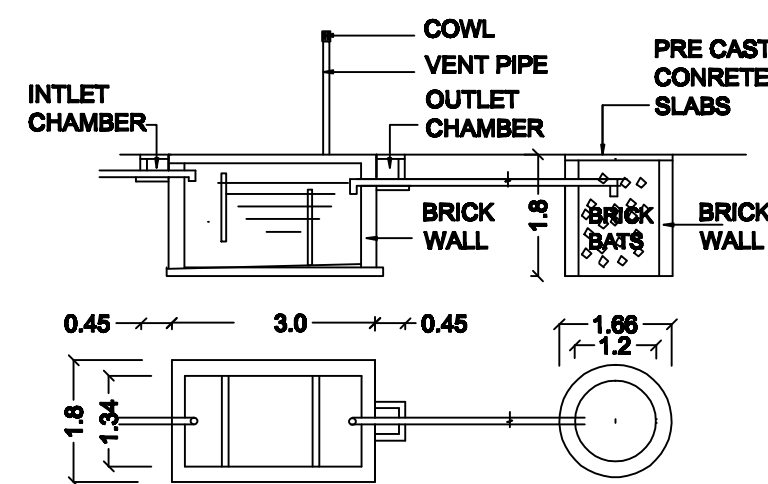
SEPTIC TANK & SOAK PIT
