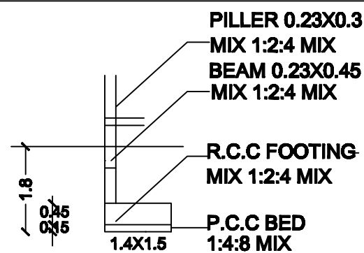
FOUNDATION DETAILS -N.T.S
