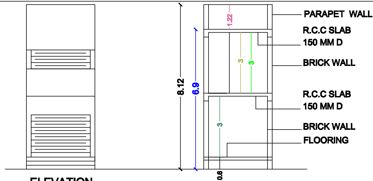
ELEVATION SECTION ON - AA S.F No:362/1M1 SAMUNDEESWARI LAND
