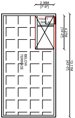
PRO. FIRST FLOOR PLAN.
