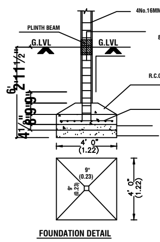
FOUNDATION DETAIL (SCALE: 1:50)
