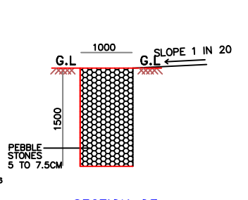
SECTION OF PEBBLE TRENCH
