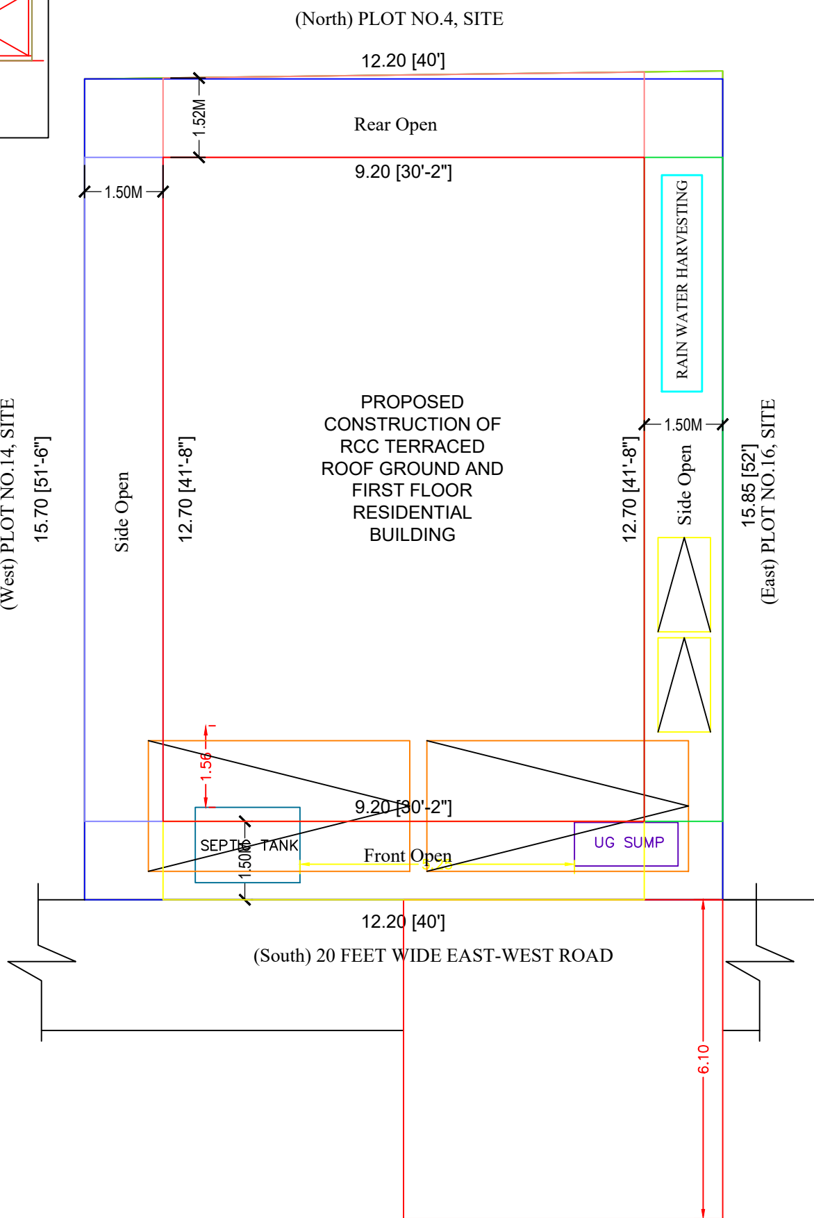
SITE PLAN
