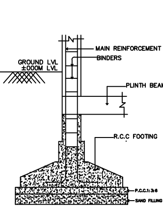
TYPICAL SECTION OF R.C.C COLUMN FOUNDATION
