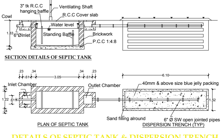
DETAILS OF SEPTIC TANK & DISPERSION TRENCH
