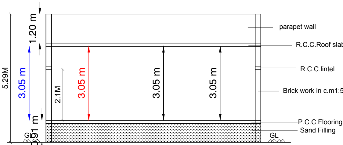
SECTION-"SR"
