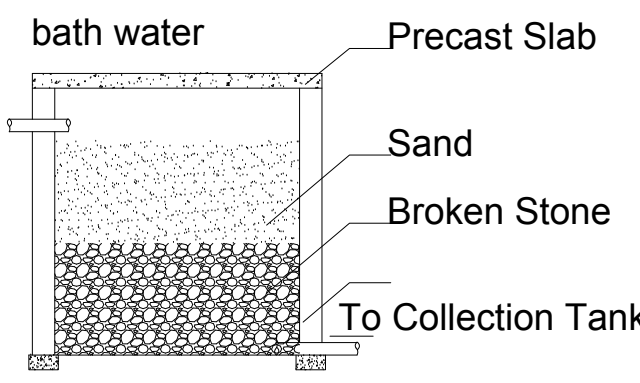
Section of Filter Unit
