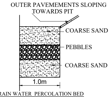
RAIN WATER PERCOLATION BED
