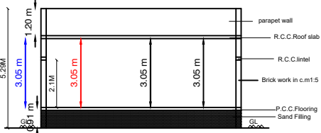
SECTION-"SR"
