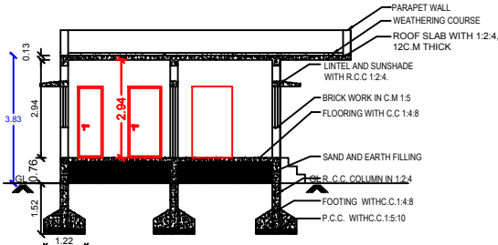
SECTION ON "AB" (NORTH) SURVEY No.117/4, LAND
