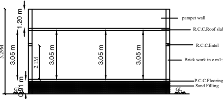
SECTION-"SR"
