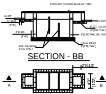
PLAN OF SEPTIC TANK
