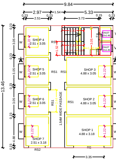
GROUND FLOOR PLAN (WEST FACING)
