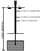
BORE WELL
