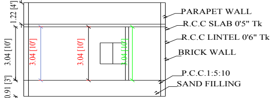
SECTION ON"AB"
