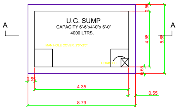
SUMP DETAIL
