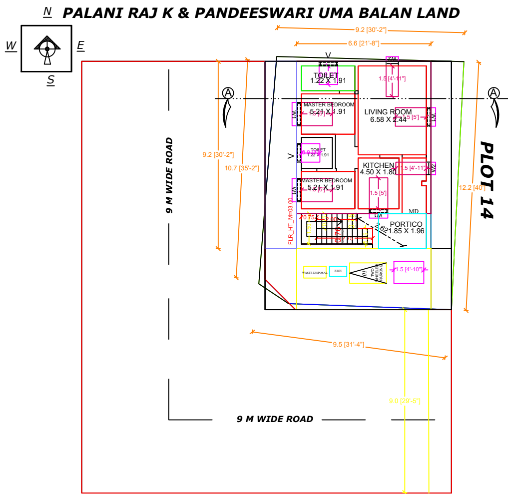
SITE CUM PRO. GROUND FLOOR PLAN
