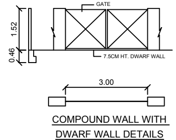
COMPOUND WALL WITH DWAFF WALL DETAILS
