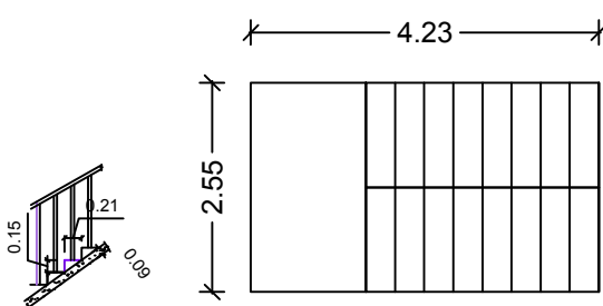
STAIRCASE DETAILS
