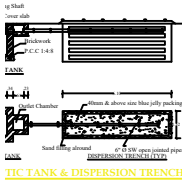
TIC TANK & DISPERSION TRENCH
