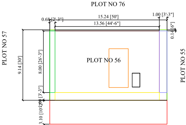
SITE PLAN
