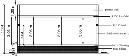
SECTION-"SR"
