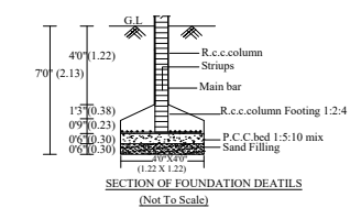
SECTION OF FOUNDATION DETAILS [Not To Scale]
