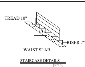
STAIRCASE DETAILS [N.T.S.]
