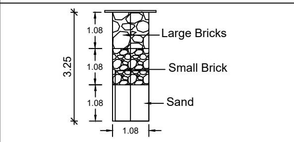
SECTION OF RAIN WATER COLLECTION PITS (NTS)
