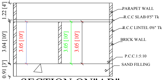
SECTION ON"AB"
