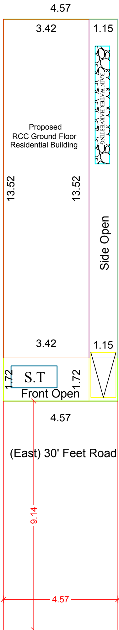
SITE PLAN
