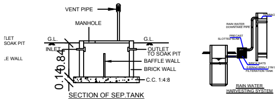
SEPTIC TANK
