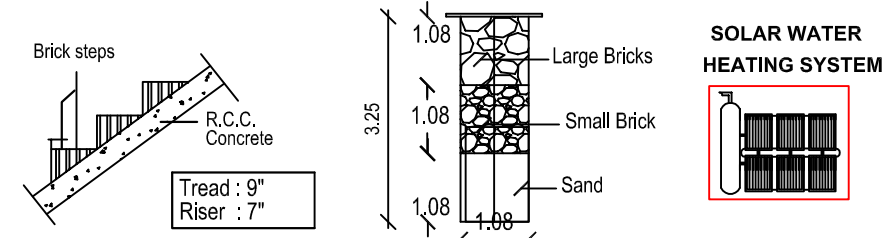
STAIRCASE DETAILS
