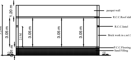
SECTION-"SR"
