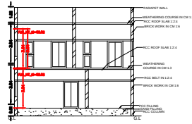
SECTION ON-AA&BB
