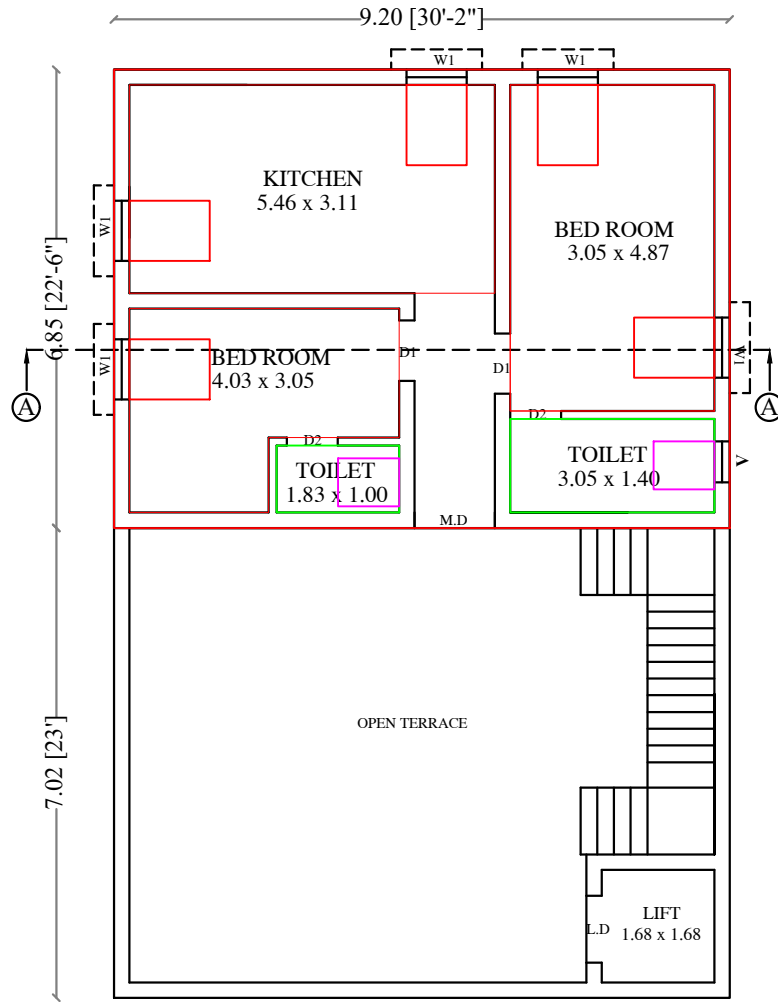
PROPOSED SECOND FLOOR
