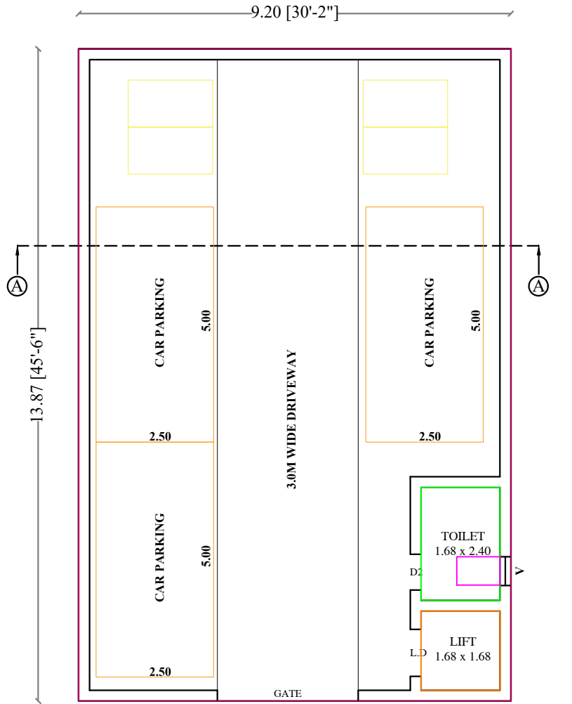
POSED GROUND FLOOR
