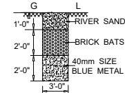
RAIN WATER PERCOLATION PIT (NTS)
