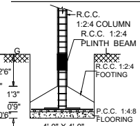
FOUNDATION DETAIL
