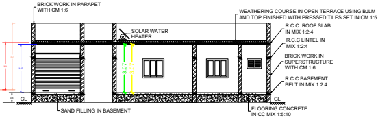
SECTION ON A-A
