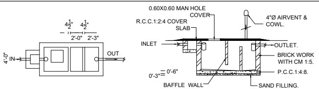
SEPTIC TANK DETAIL
