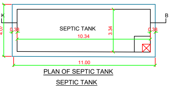
SEPTIC TANK
