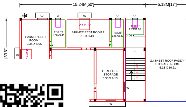
ND FLOOR PLAN (AST FACING)
