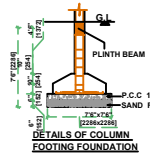
DETAILS OF COLUMN FOOTING FOUNDATION
