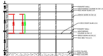
SECTION ON-AA&amp;BB
