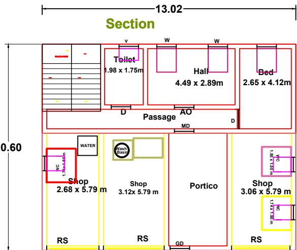
EX GROUND FLOOR PLAN
