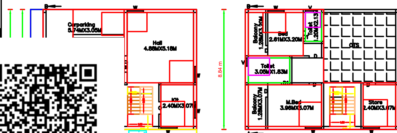
FIRST FLOOR PLAN(Pro.)
