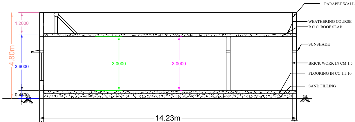
SECTION AB
