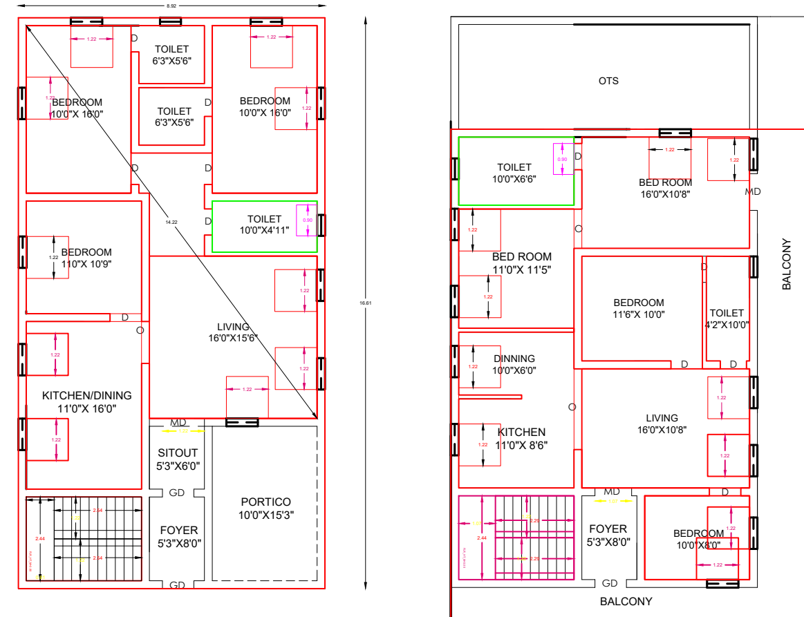
GROUND FLOOR PLAN [EAST FACING]
