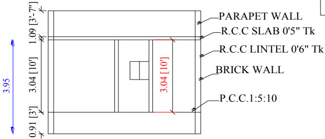
SECTION ON"AB"
