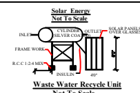
Waste Water Recycle Unit
