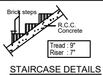
STAIRCASE DETAILS
