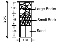
SECTION OF RAIN WATER COLLECTION PITS (NTS)
