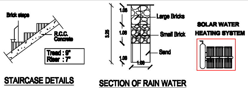
SECTION OF RAIN WATER
