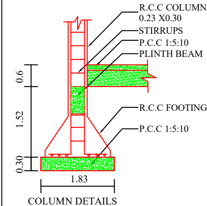
COLUMN DETAILS
