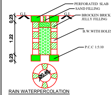
RAIN WATERPERCOLATION
