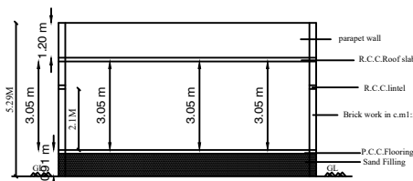
SECTION-"SR"
