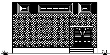
FRONT ELEVATION
