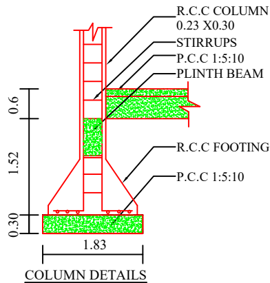
COLUMN DETAILS
