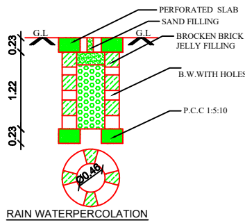
RAIN WATERPERCOLATION
