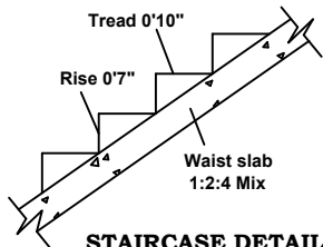
STAIRCASE DETAILS (NOT TO SCALE)
